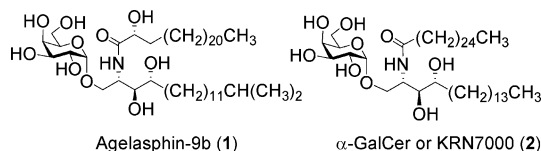
Figure 1. \alpha -Glycosphingolipids.
